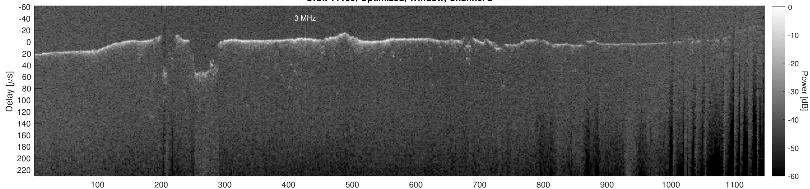
Orbit 11136, Cluttergram
