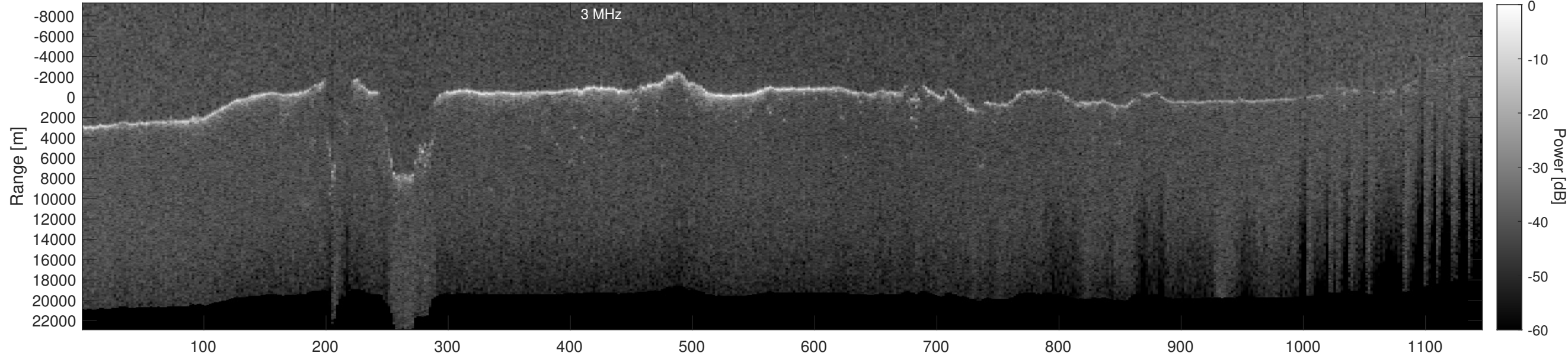
Orbit 11136, Depth-Corrected Cluttergram
