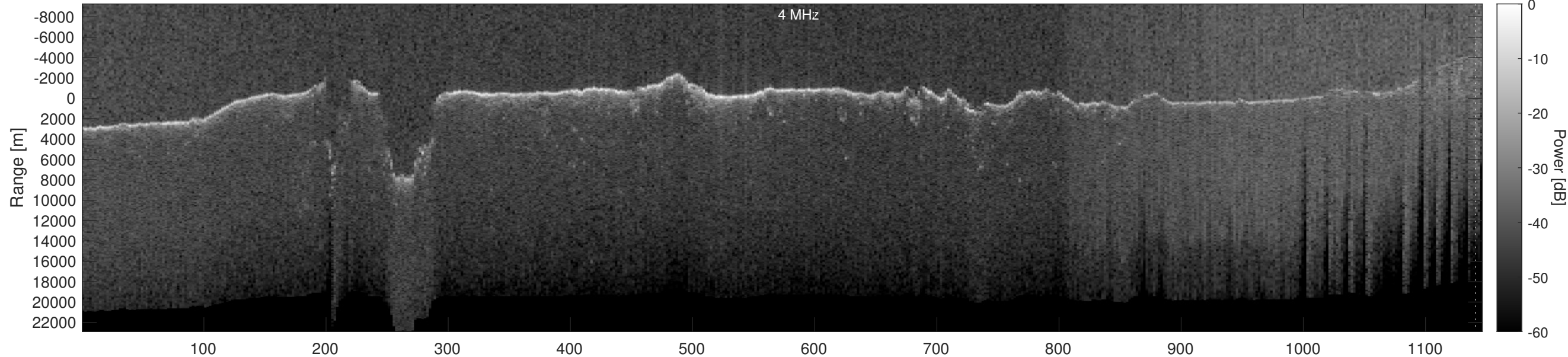
Orbit 11136, Optimized, Window, Depth-Corrected, Channel 2
