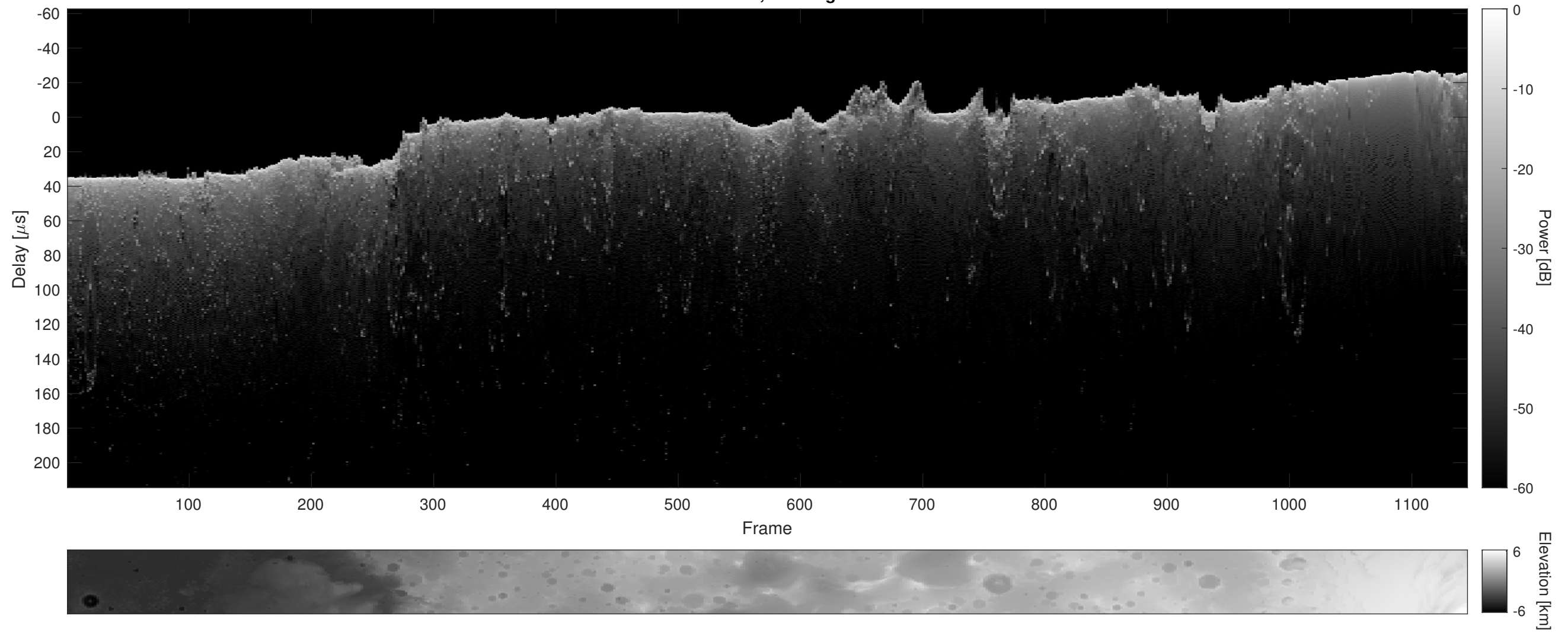
Orbit 11137, Cluttergram
