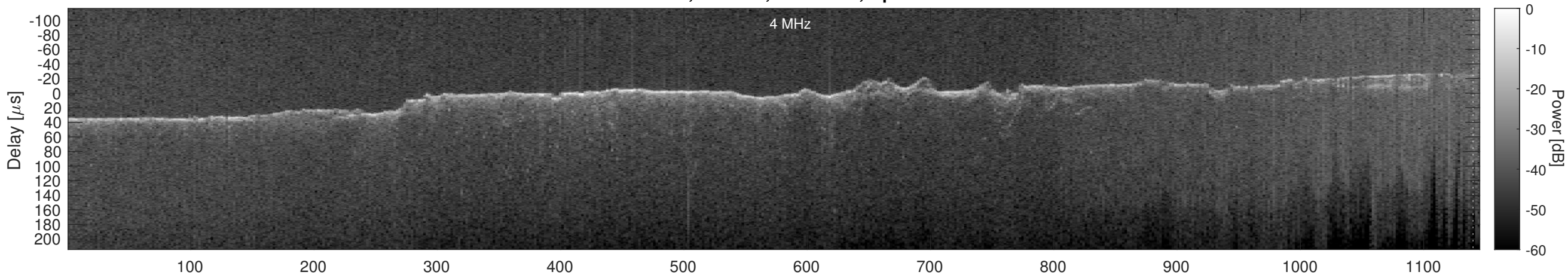
Orbit 11137, Cluttergram
