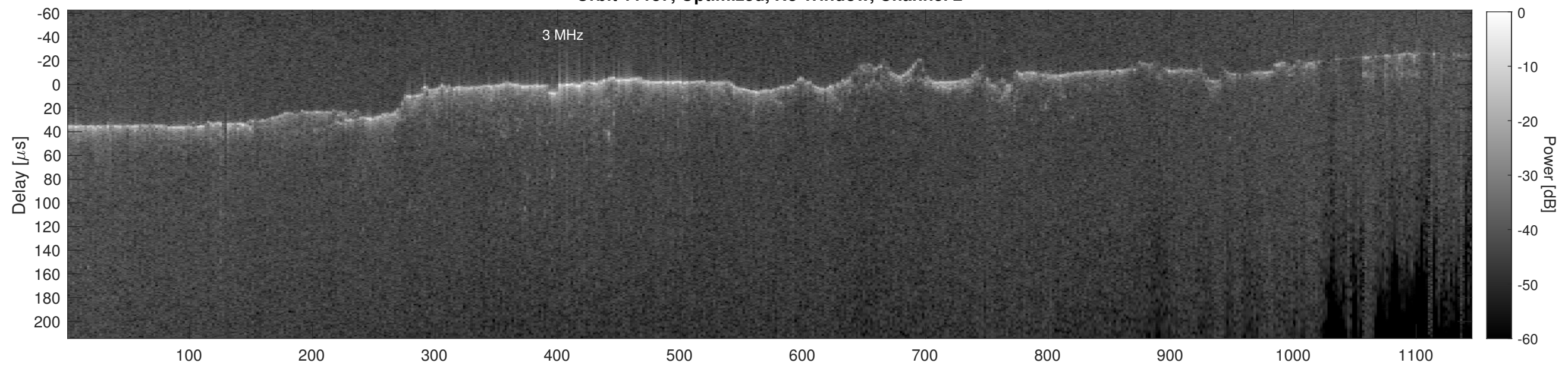
Orbit 11137, Cluttergram
