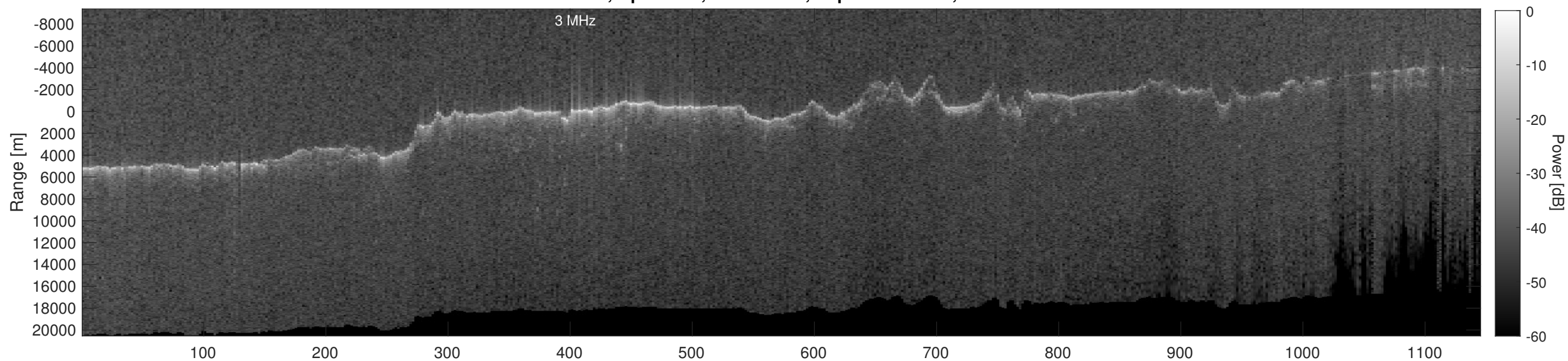
Orbit 11137, Depth-Corrected Cluttergram
