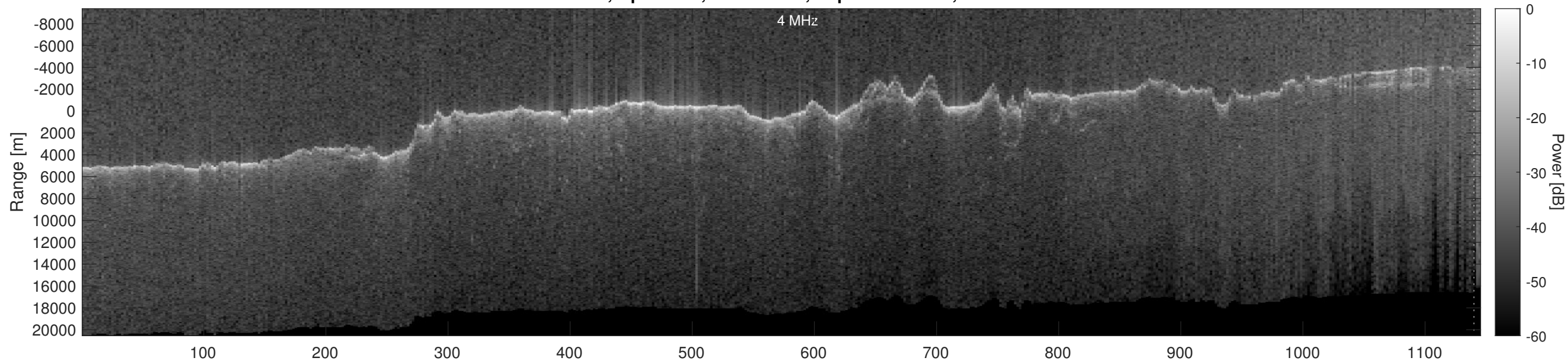
Orbit 11137, Optimized, No Window, Depth-Corrected, Channel 2
