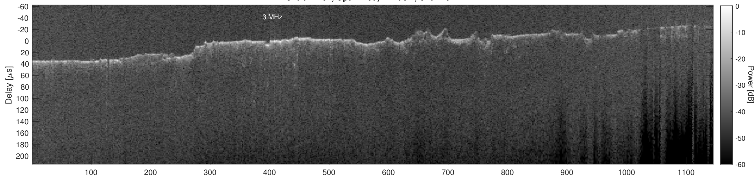
Orbit 11137, Cluttergram
