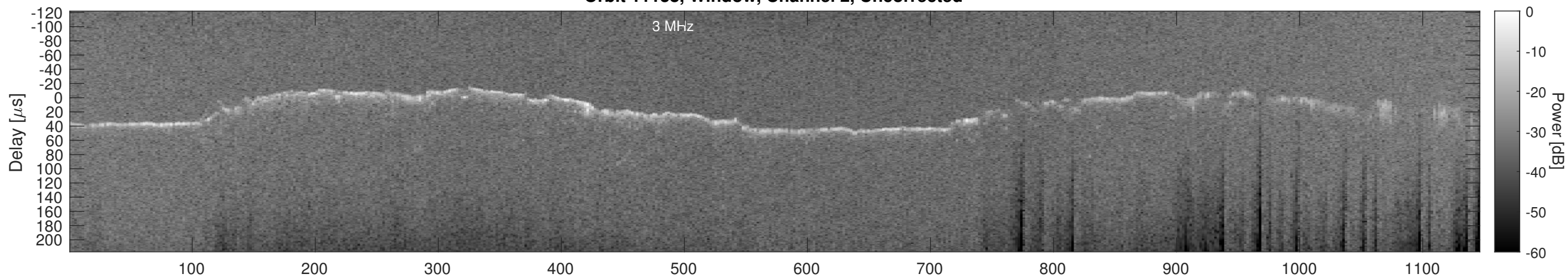
Orbit 11138, Window, Channel 2, Chapman
