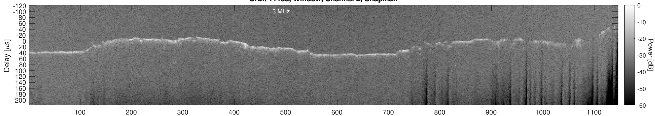
Orbit 11138, Window, Channel 2, Optimized
