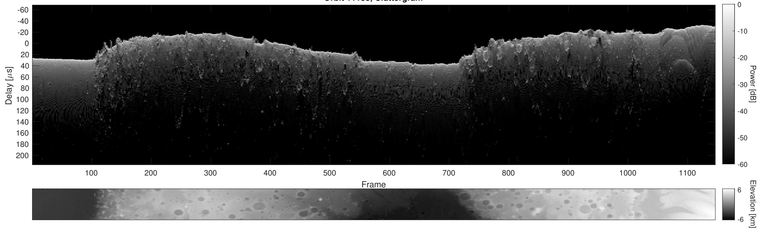
Orbit 11138, Cluttergram
