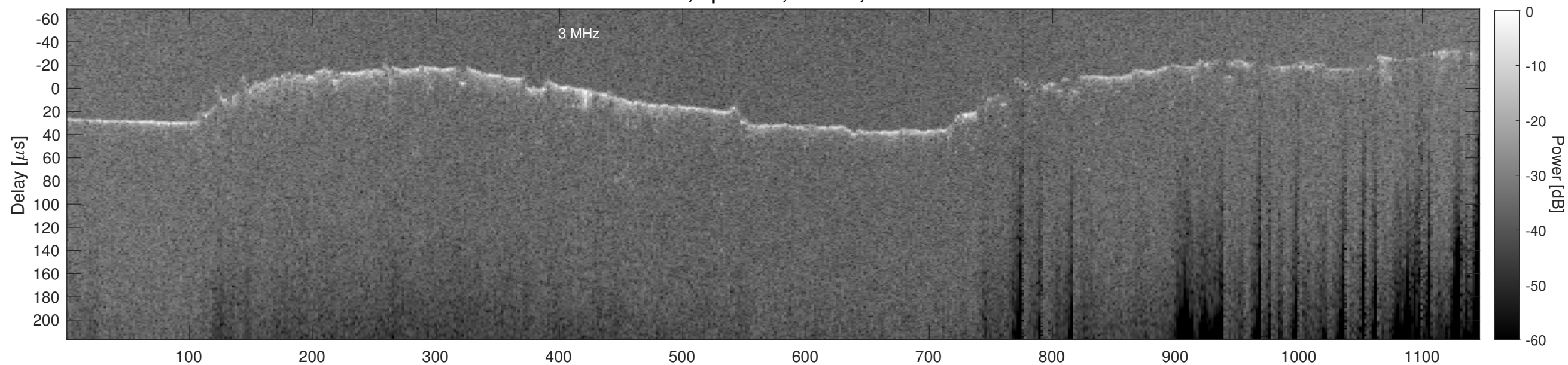
Orbit 11138, Cluttergram
