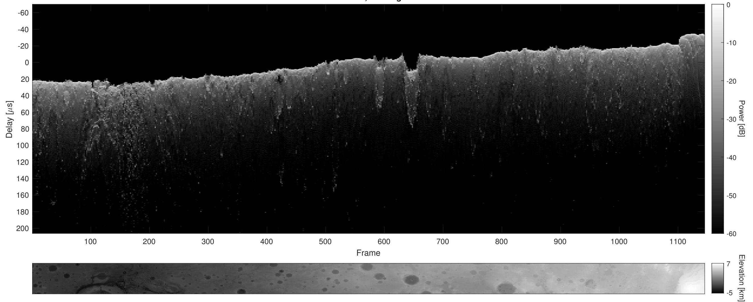
Orbit 11139, Cluttergram
