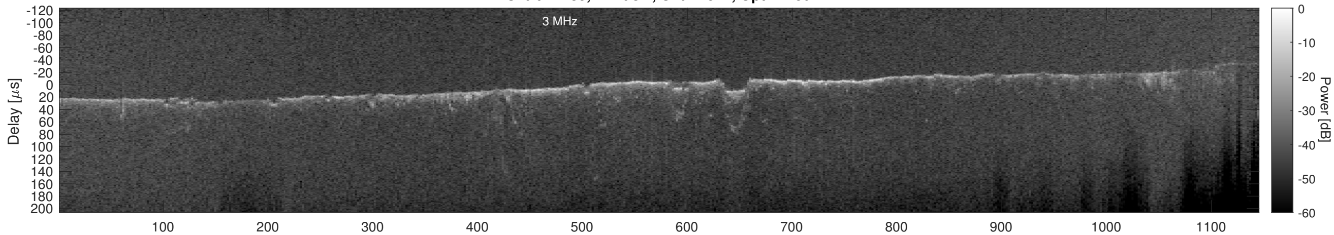
Orbit 11139, Cluttergram
