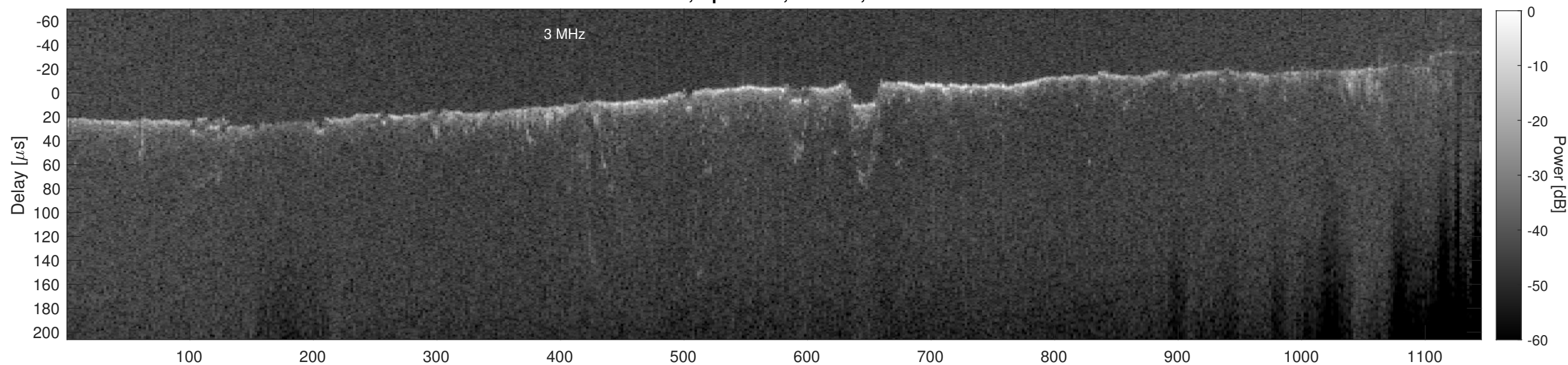
Orbit 11139, Cluttergram
