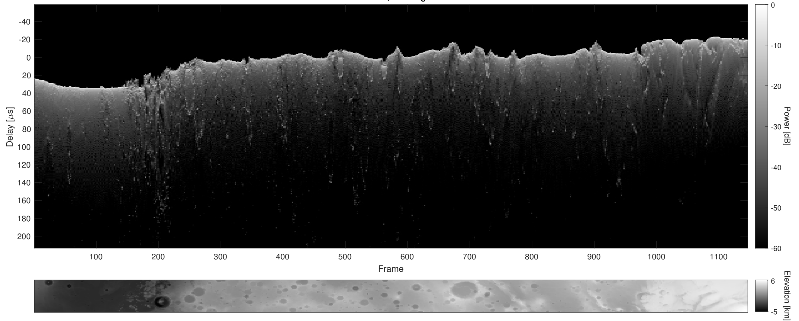
Orbit 11141, Cluttergram
