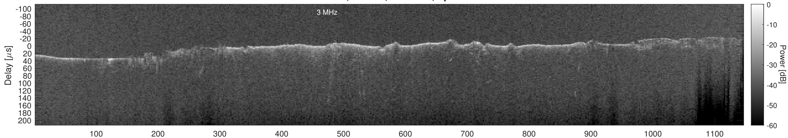
Orbit 11141, Cluttergram
