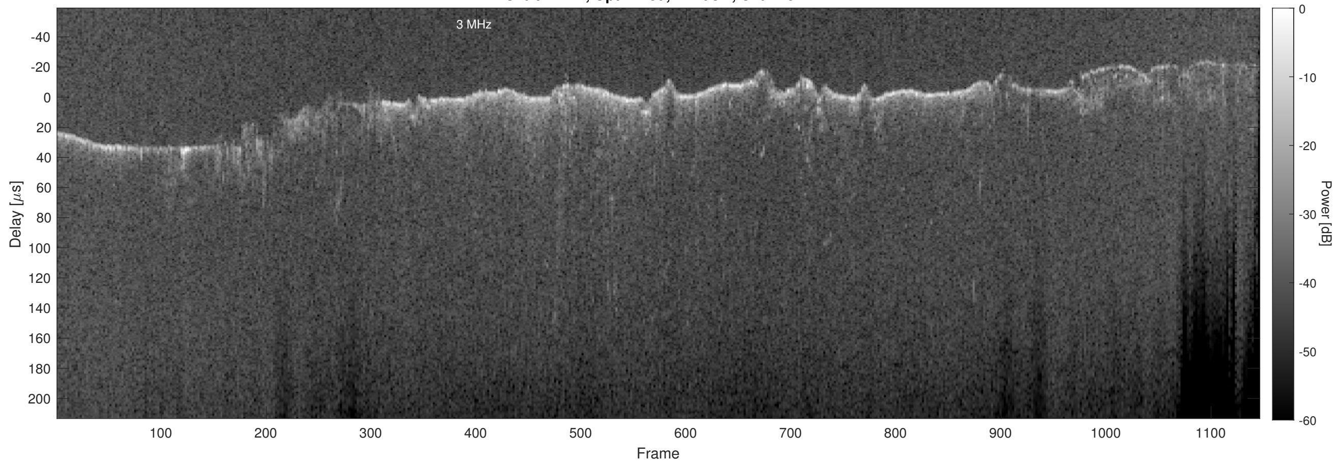
Orbit 11141, Optimized, Window, Channel 2
