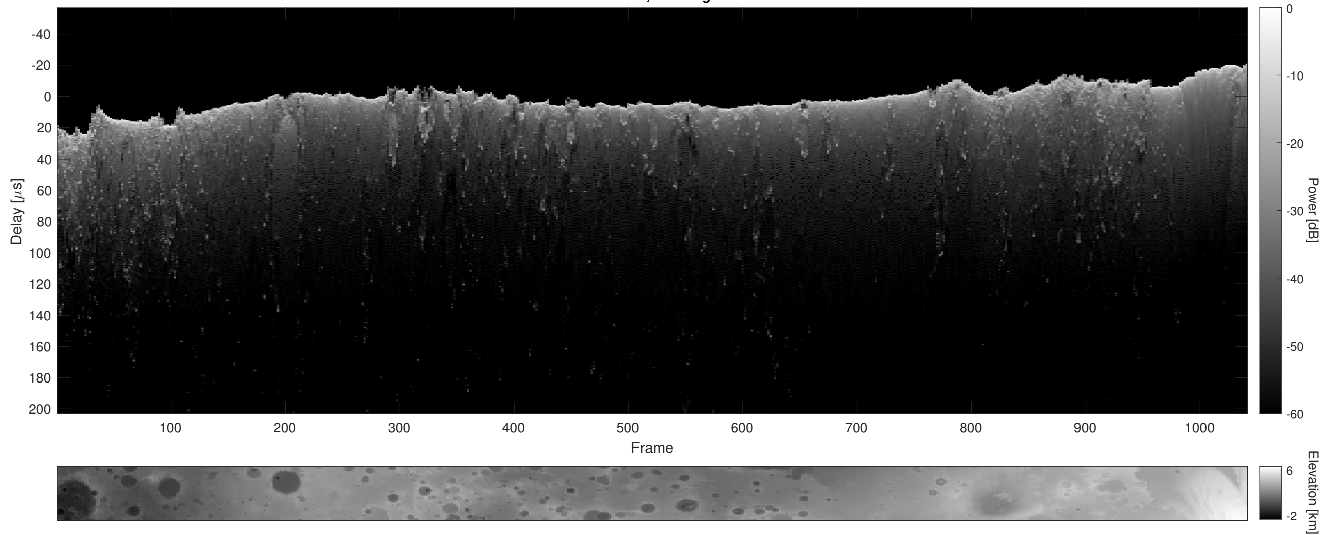
Orbit 11142, Cluttergram
