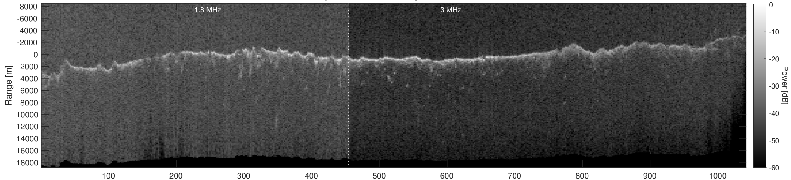
Orbit 11142, Depth-Corrected Cluttergram
