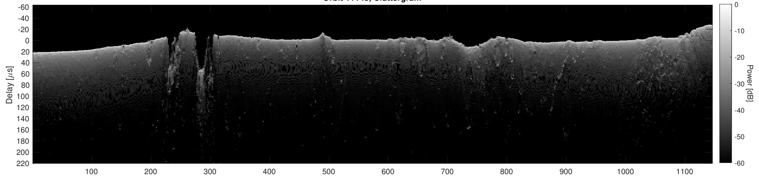
Orbit 11143, Cluttergram
