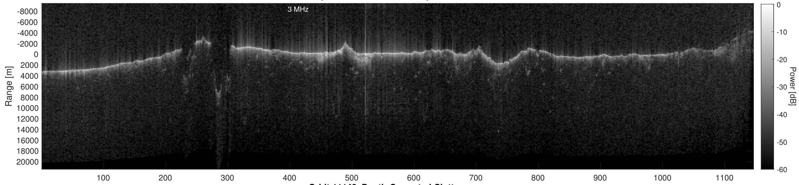
Orbit 11143, Depth-Corrected Cluttergram
