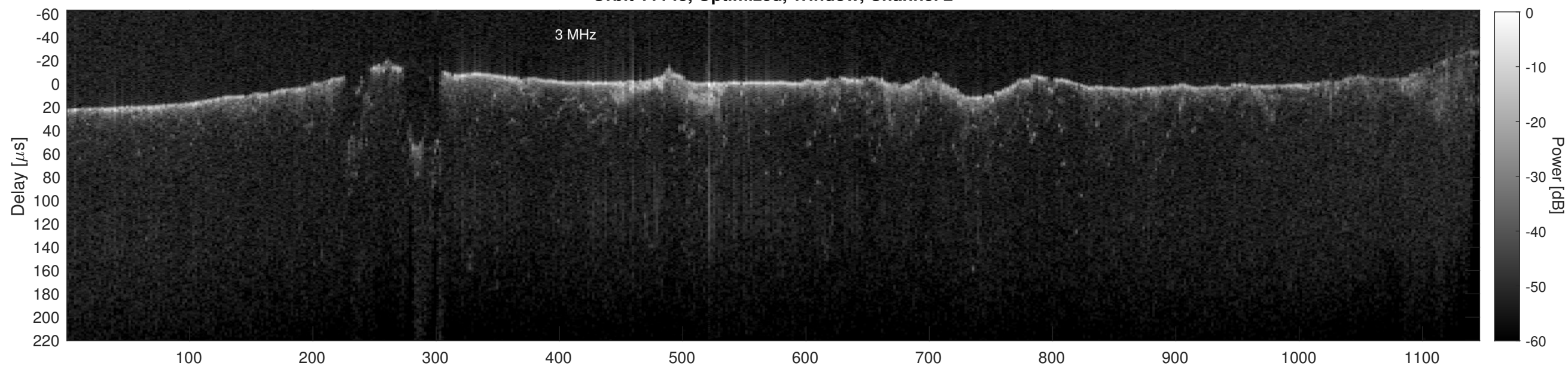
Orbit 11143, Cluttergram
