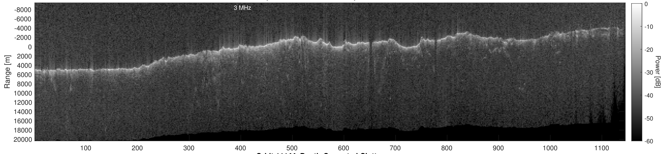
Orbit 11144, Depth-Corrected Cluttergram
