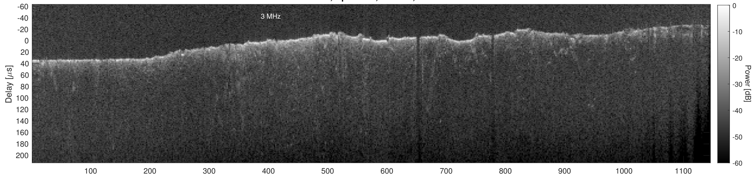
Orbit 11144, Cluttergram
