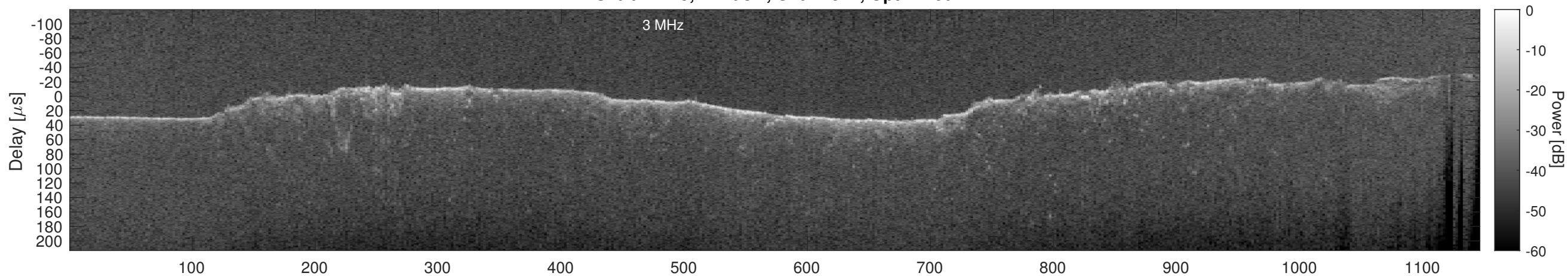
Orbit 11145, Cluttergram
