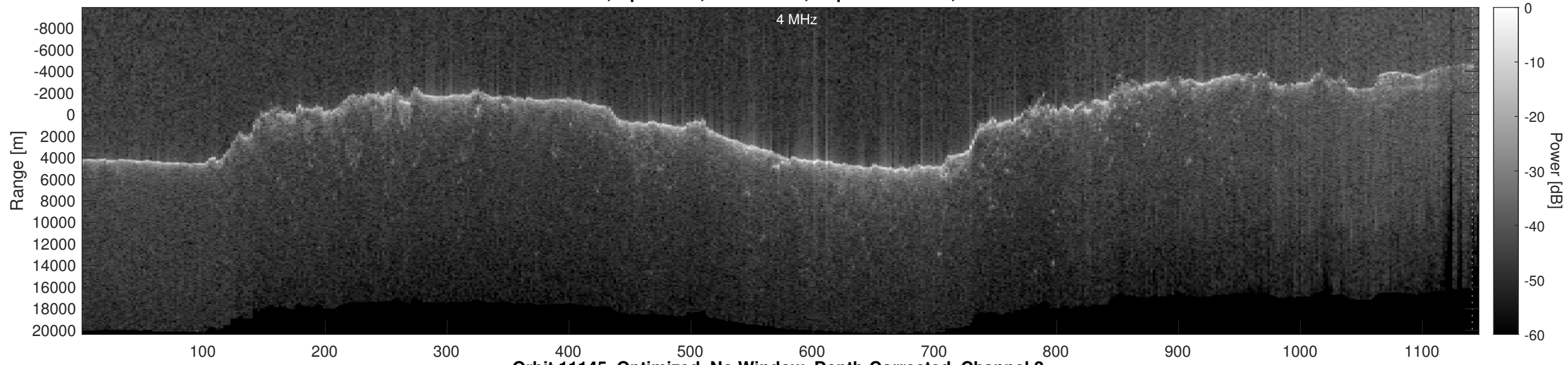
Orbit 11145, Optimized, No Window, Depth-Corrected, Channel 2
