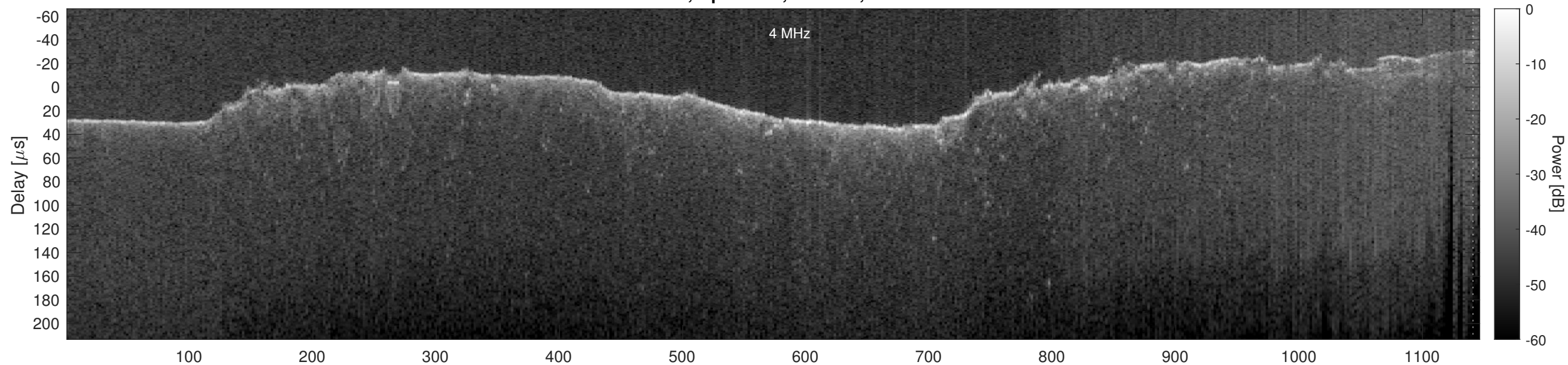
Orbit 11145, Optimized, Window, Channel 2
