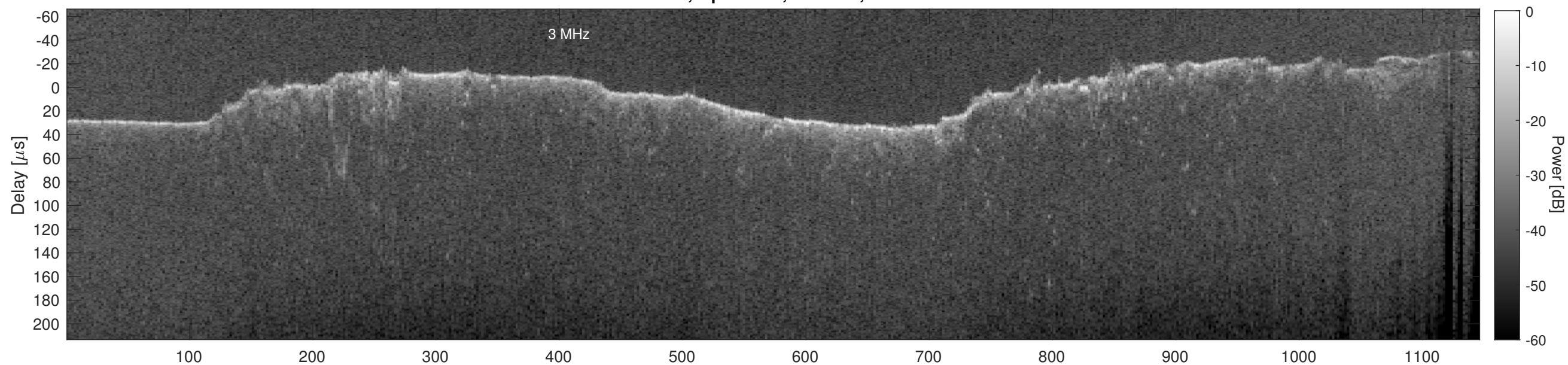
Orbit 11145, Cluttergram
