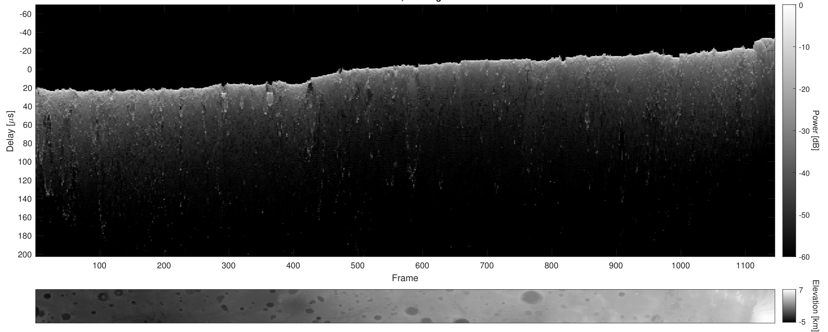
Orbit 11146, Cluttergram
