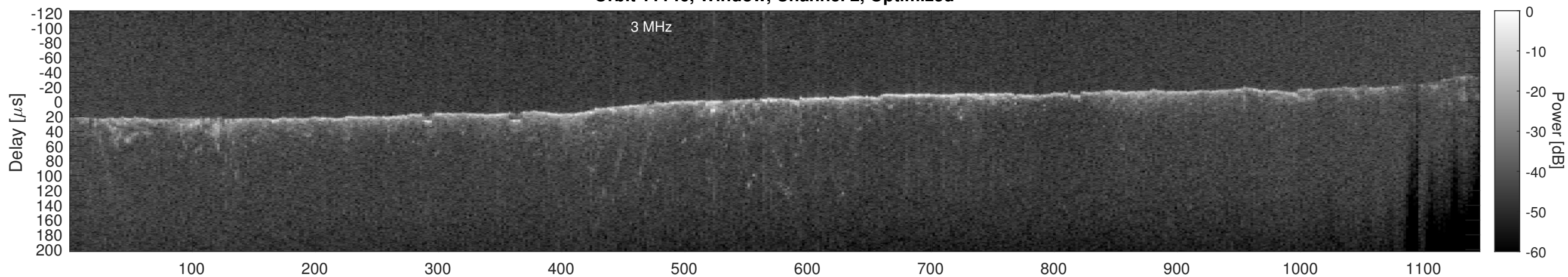
Orbit 11146, Cluttergram
