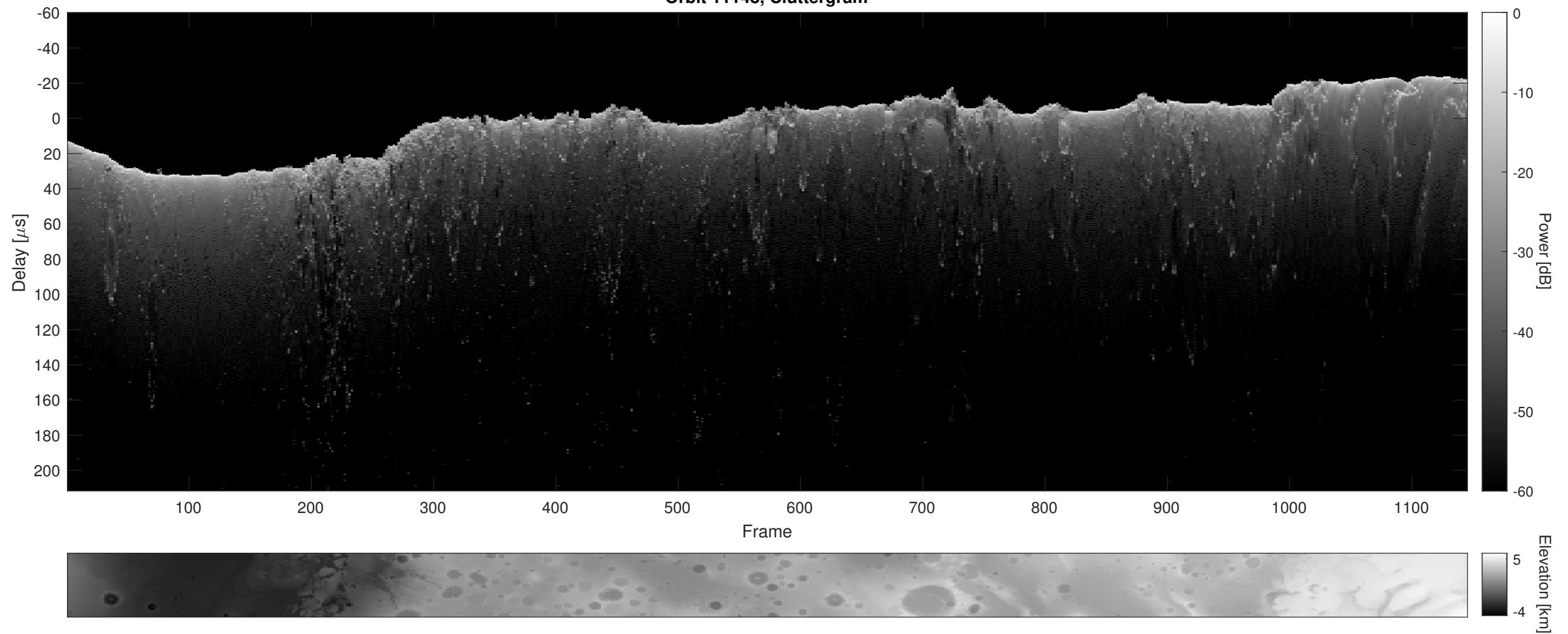
Orbit 11148, Cluttergram
