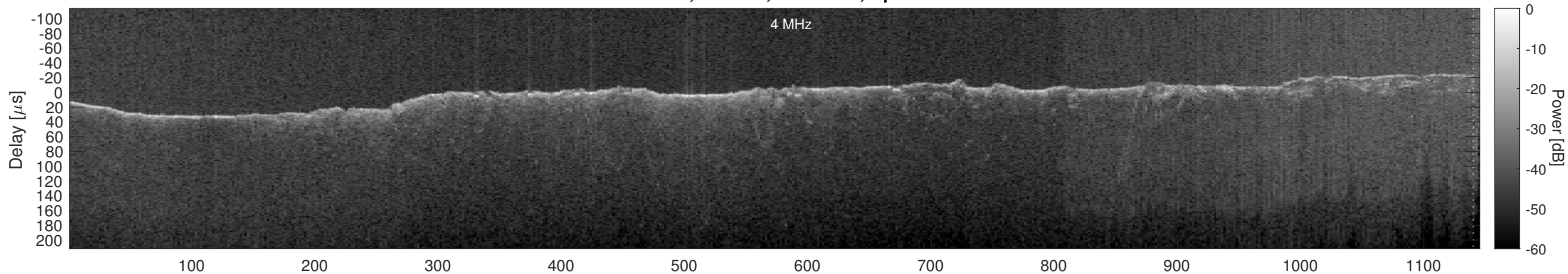
Orbit 11148, Cluttergram
