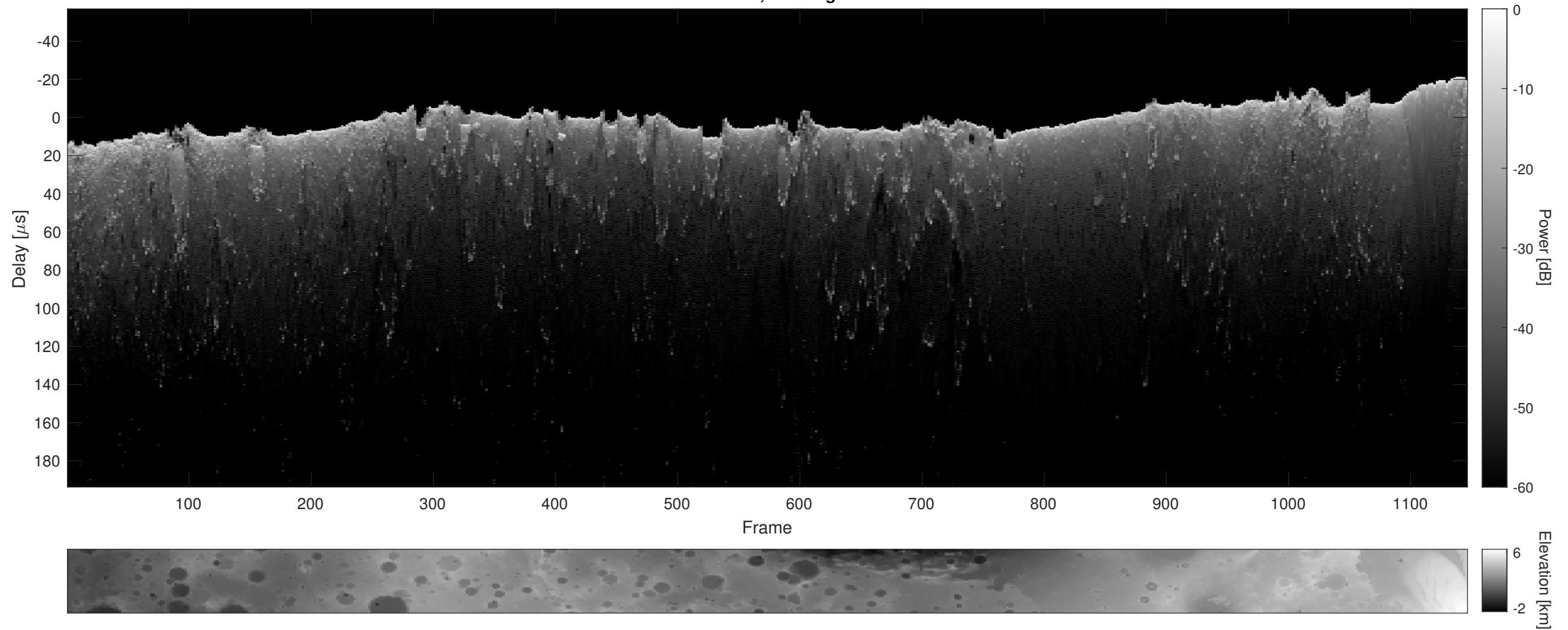
Orbit 11149, Cluttergram
