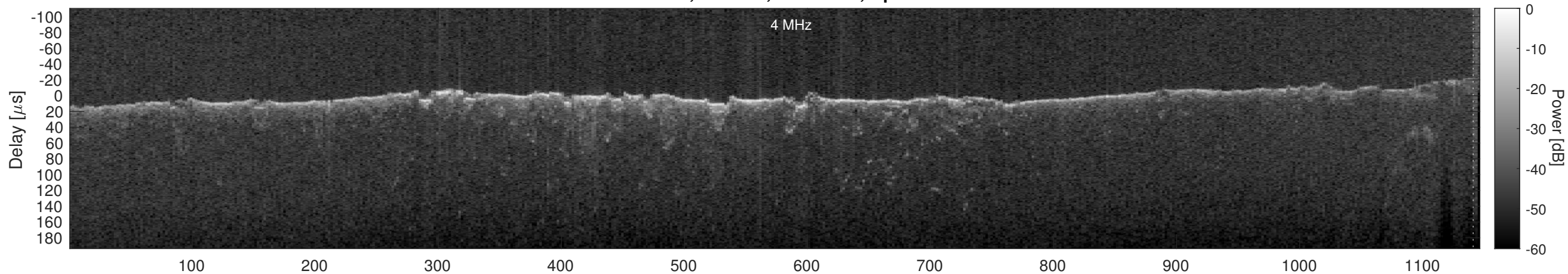
Orbit 11149, Cluttergram
