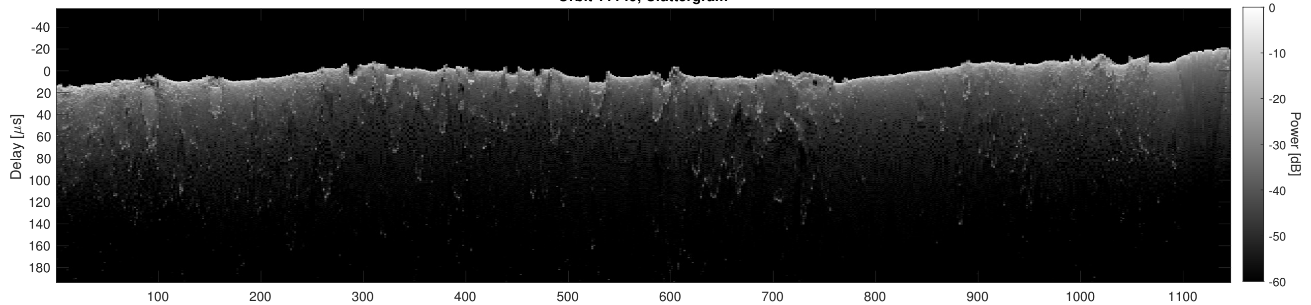
Orbit 11149, Cluttergram
