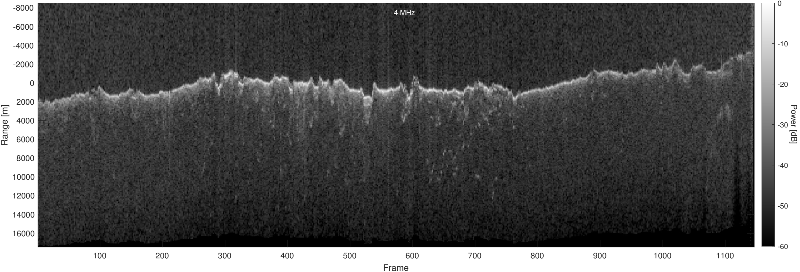
Orbit 11149, Optimized, Window, Depth-Corrected, Channel 2
