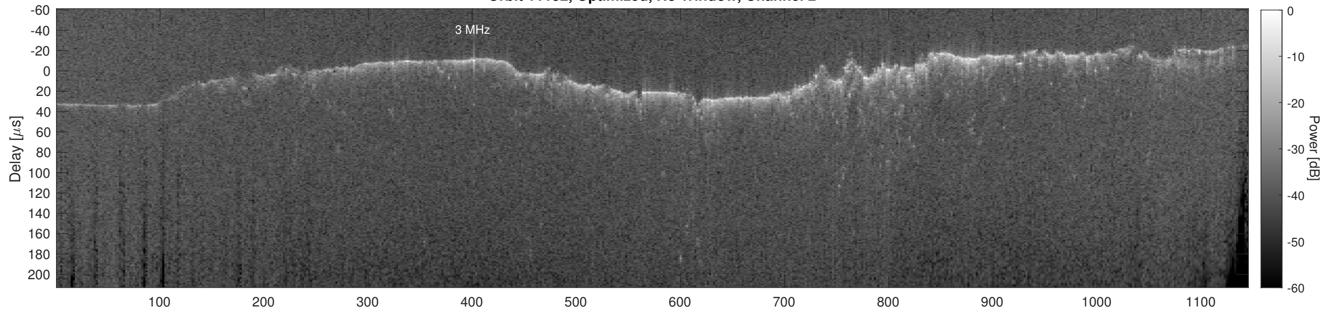
Orbit 11152, Cluttergram
