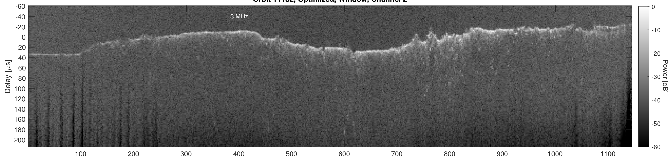
Orbit 11152, Cluttergram
