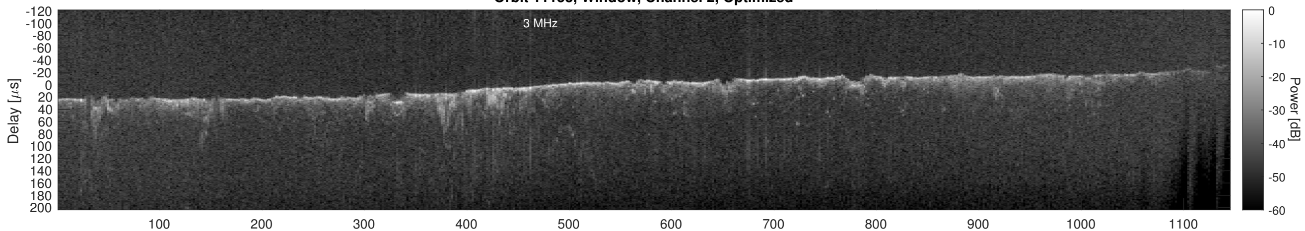
Orbit 11153, Cluttergram
