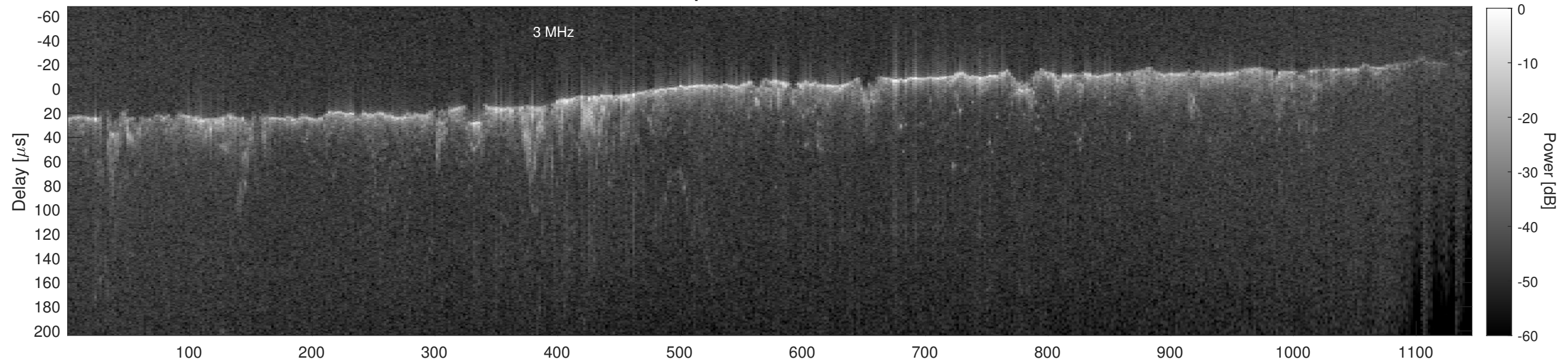
Orbit 11153, Cluttergram
