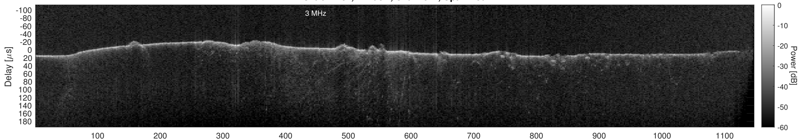
Orbit 11154, Cluttergram
