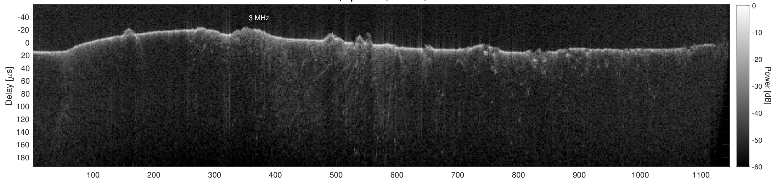
Orbit 11154, Cluttergram
