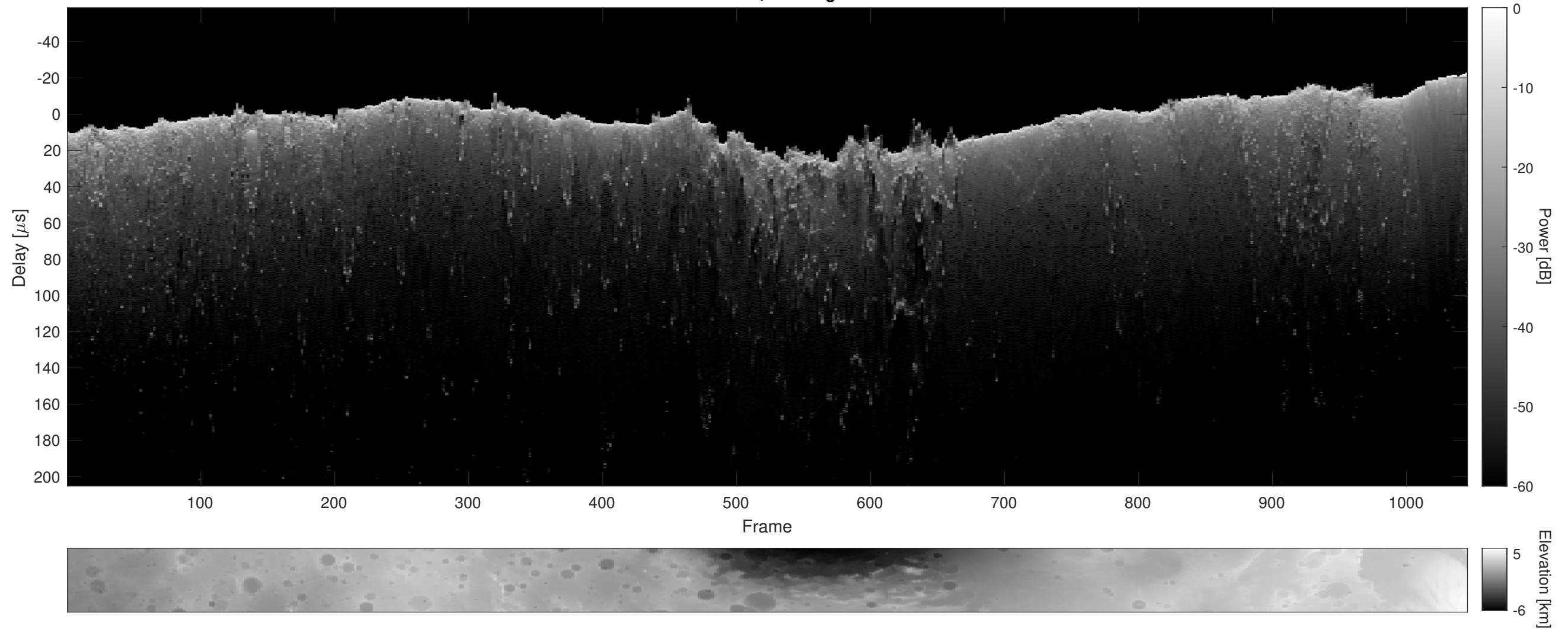
Orbit 11156, Cluttergram
