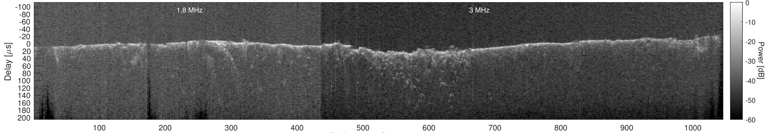
Orbit 11156, Cluttergram
