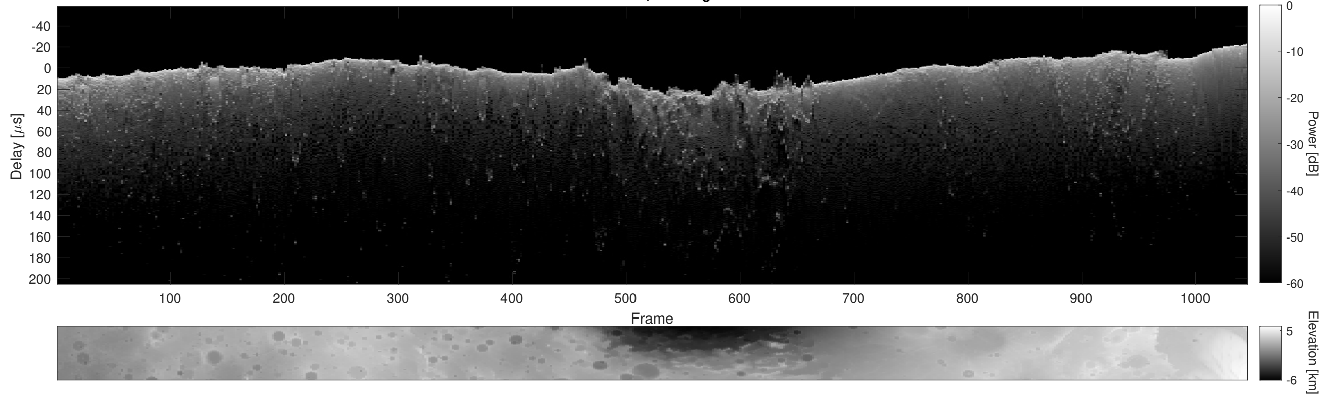
Orbit 11156, Cluttergram
