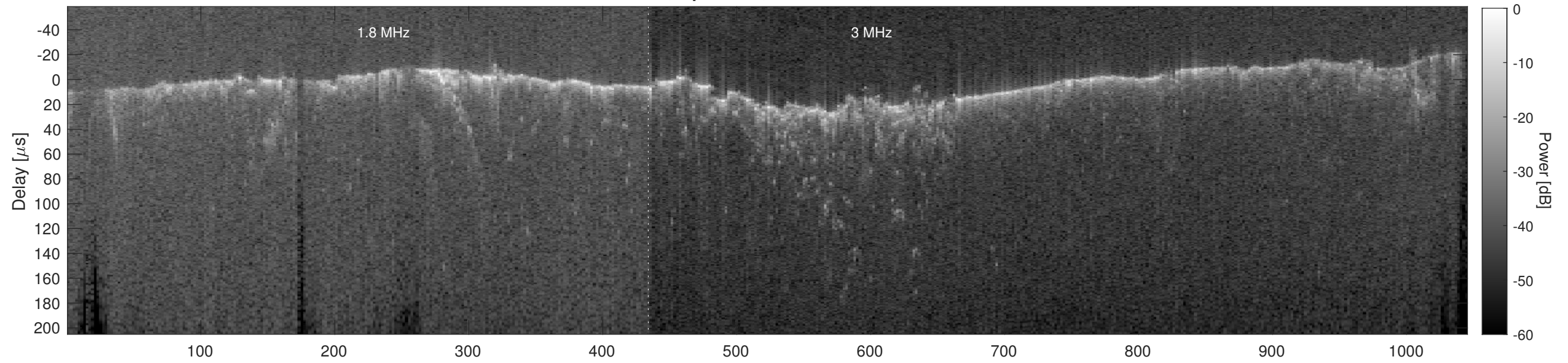
Orbit 11156, Cluttergram
