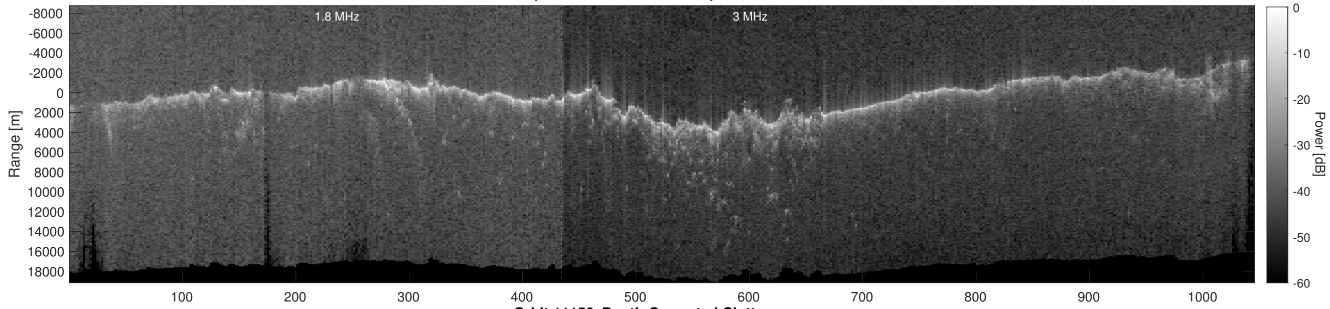
Orbit 11156, Depth-Corrected Cluttergram
