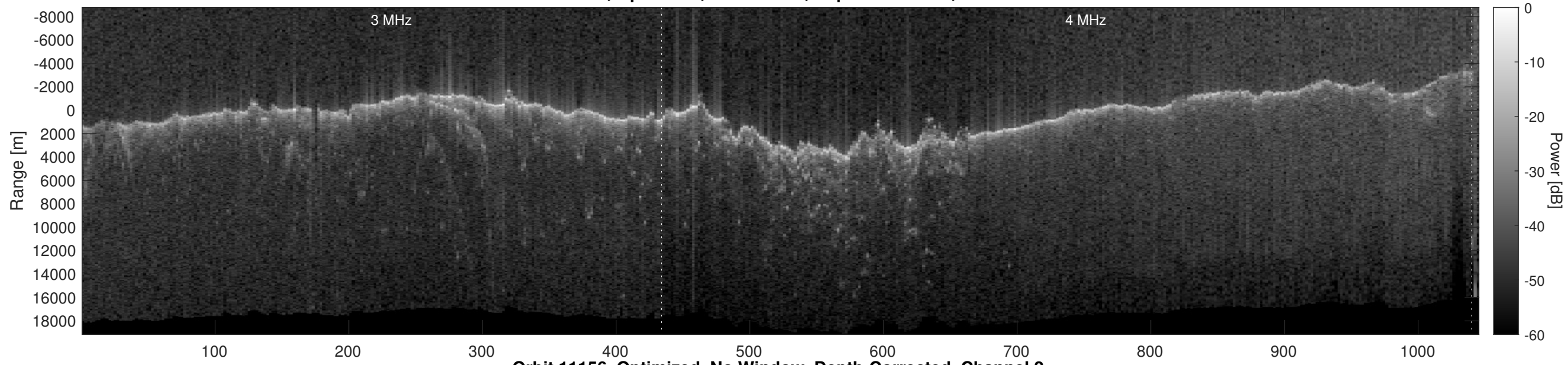
Orbit 11156, Optimized, No Window, Depth-Corrected, Channel 2
