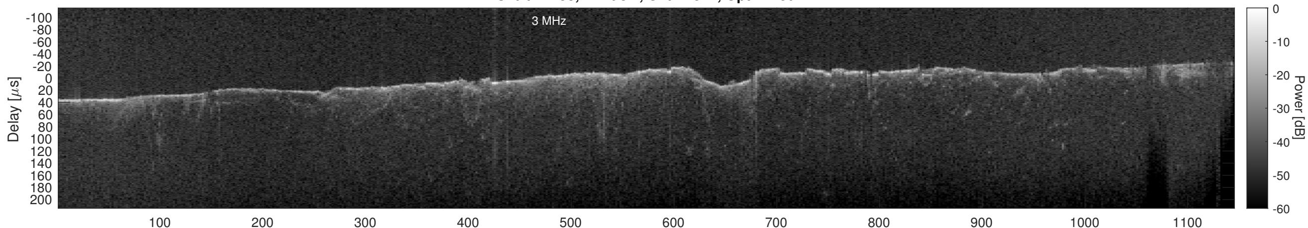
Orbit 11158, Cluttergram
