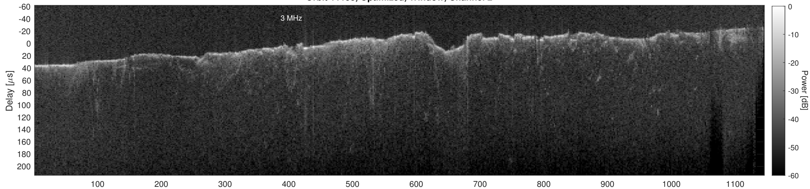
Orbit 11158, Cluttergram
