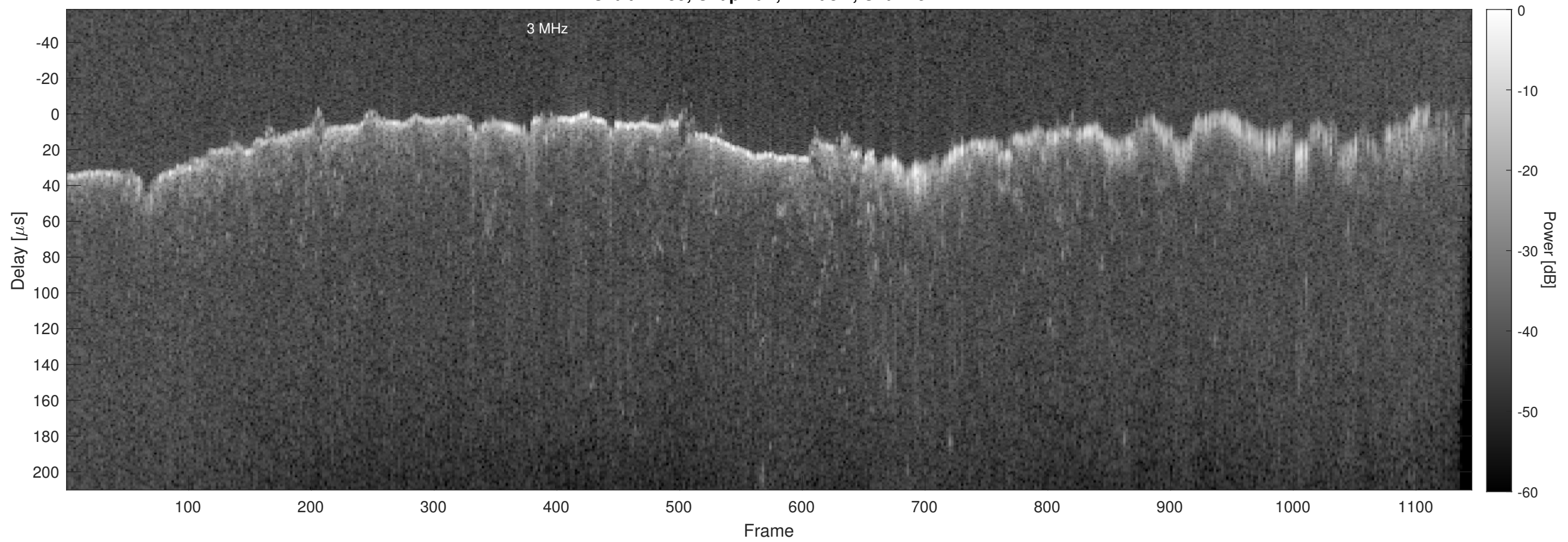
Orbit 11159, Chapman, Window, Channel 2
