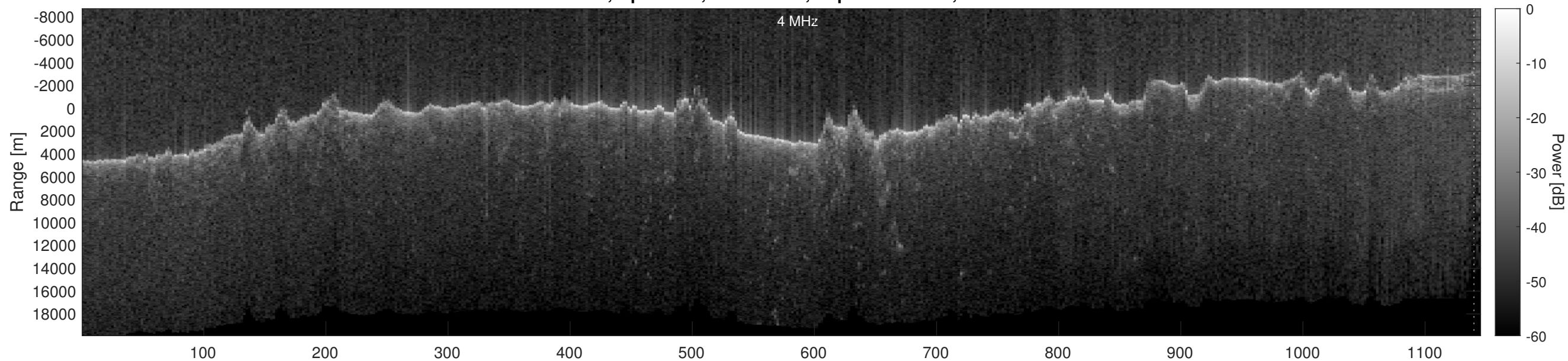
Orbit 11159, Optimized, No Window, Depth-Corrected, Channel 2
