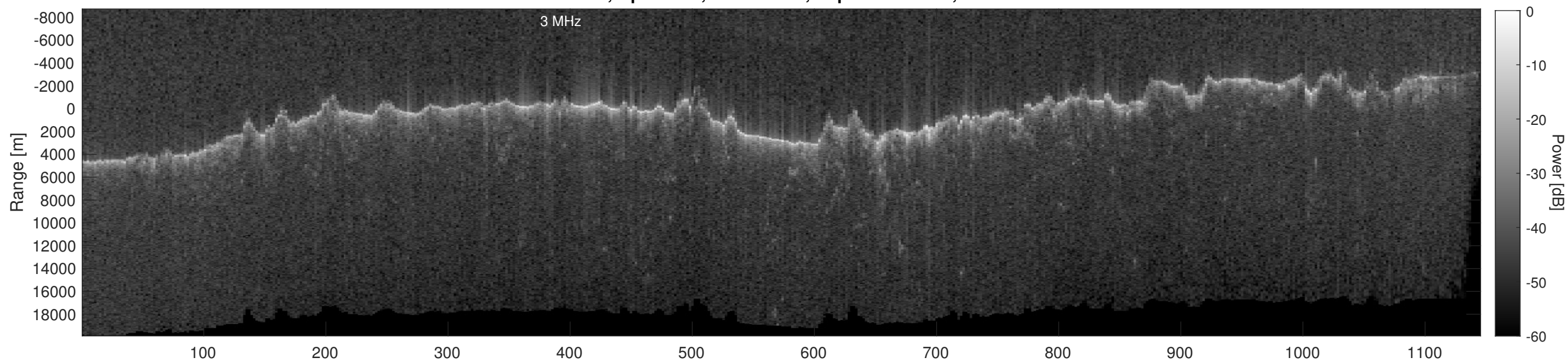
Orbit 11159, Depth-Corrected Cluttergram
