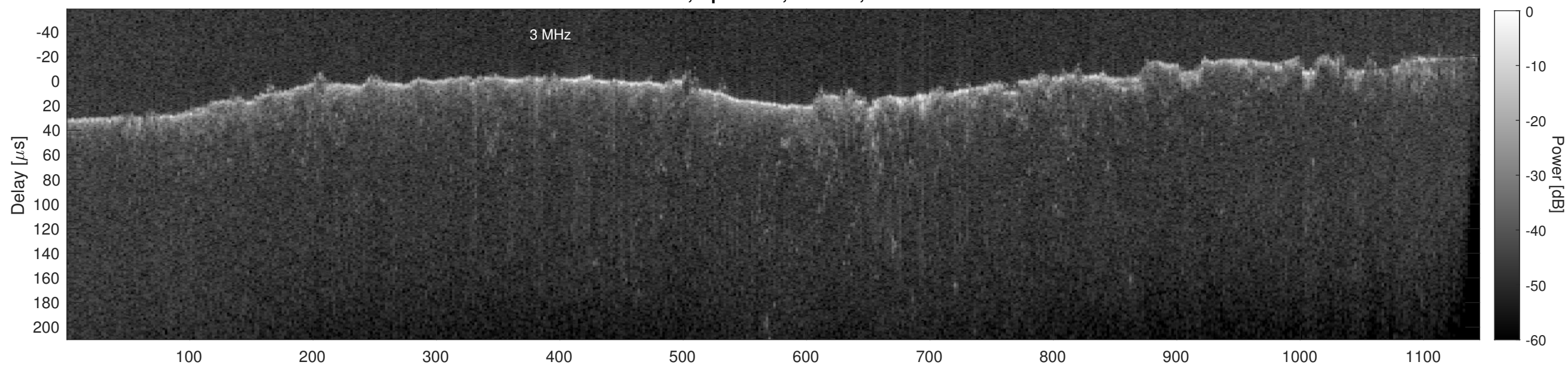
Orbit 11159, Cluttergram
