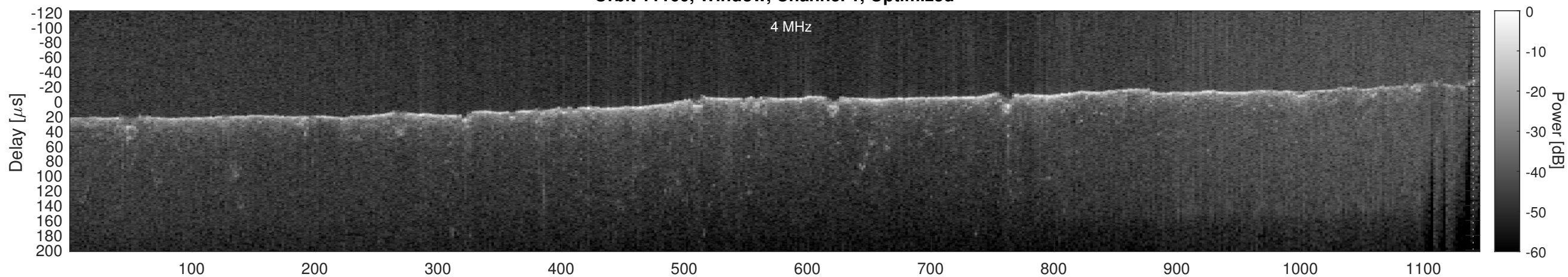
Orbit 11160, Cluttergram
