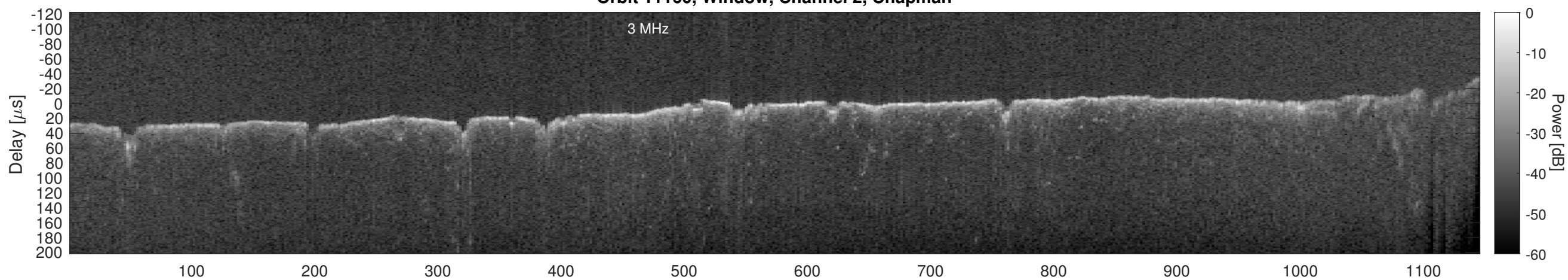
Orbit 11160, Window, Channel 2, Optimized
