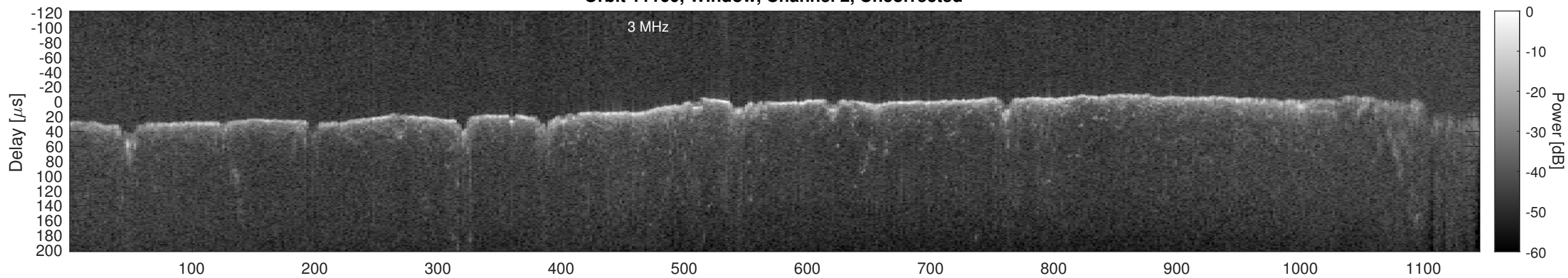
Orbit 11160, Window, Channel 2, Chapman
