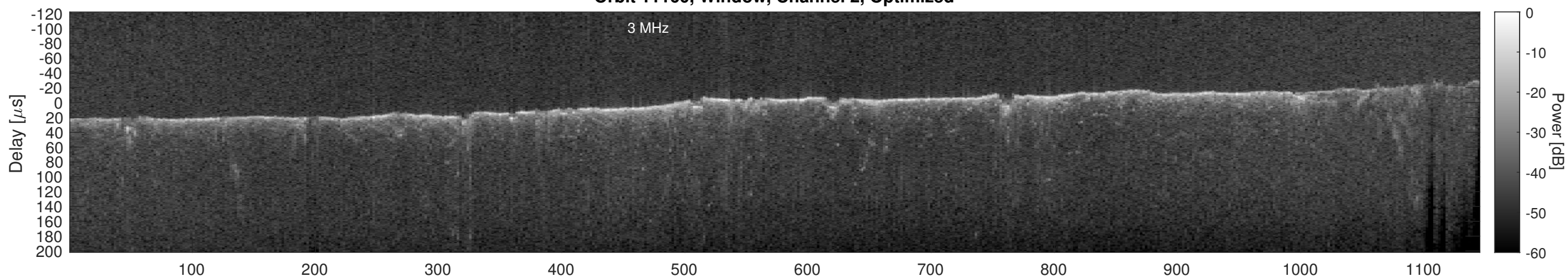
Orbit 11160, Cluttergram
